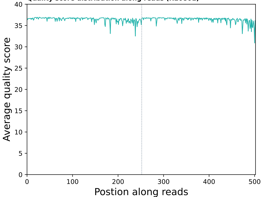
Quality score distribution along reads (R10801)
